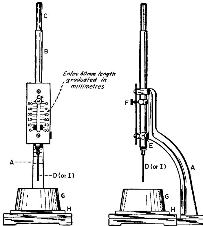
NOTE 1—Ring, G, and plate, H, are not required for this test.
